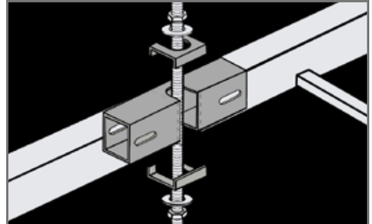
Split Splice/Hanger Coupling Part #ASP-SPLIT (hardware incl.)
