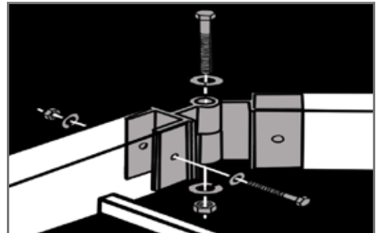
Horizontal Hinge Connector Part #AFS-HCR (hardware incl.)
