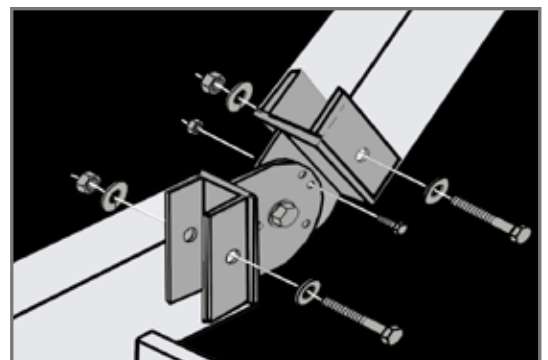
Vertical Hinge Connector Part #AFS-VCR (hardware incl.)
